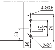
Drilling drawing for bottom pivot hinge
