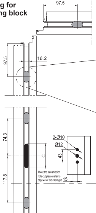
The hole-cut position of upper and lower corner device connection block on sash
