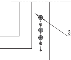
Drilling drawing for frame connecting block
