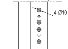
Drilling drawing for frame connecting block
