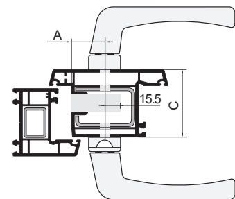
Drilling size of transmitter with key
