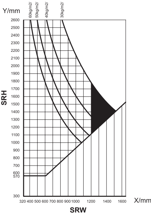
The load-bearing curve of 90kg pivot hinge
