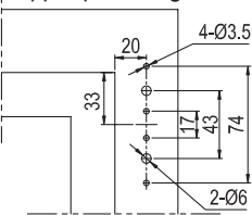
Drilling drawing for upper pivot hinge
