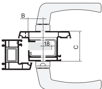
Drilling size of door lock
