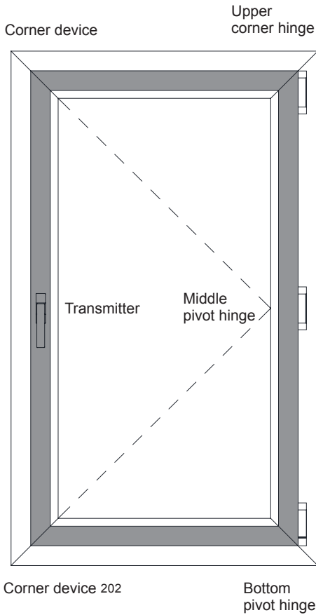
Installation position diagram of fireproof window hardware
