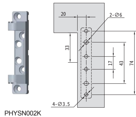
Upper pivot hinge installation instruction
