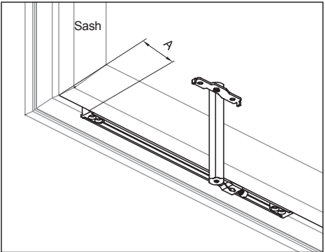
key point of installation of PFC001 series casement restrictor
