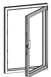
Unlock the push button, contra-rotating the handle to 180° from the locking status, then the window can be opened inward and side hung.
