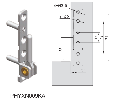
Bottom pivot hinge installation instruction
