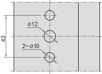
Drilling size of handle & transmitter
