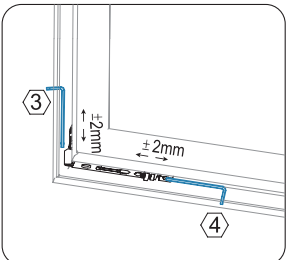
Concealed hinge installation instruction
