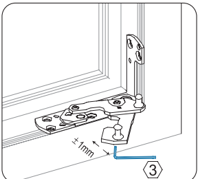
Concealed hinge installation instruction
