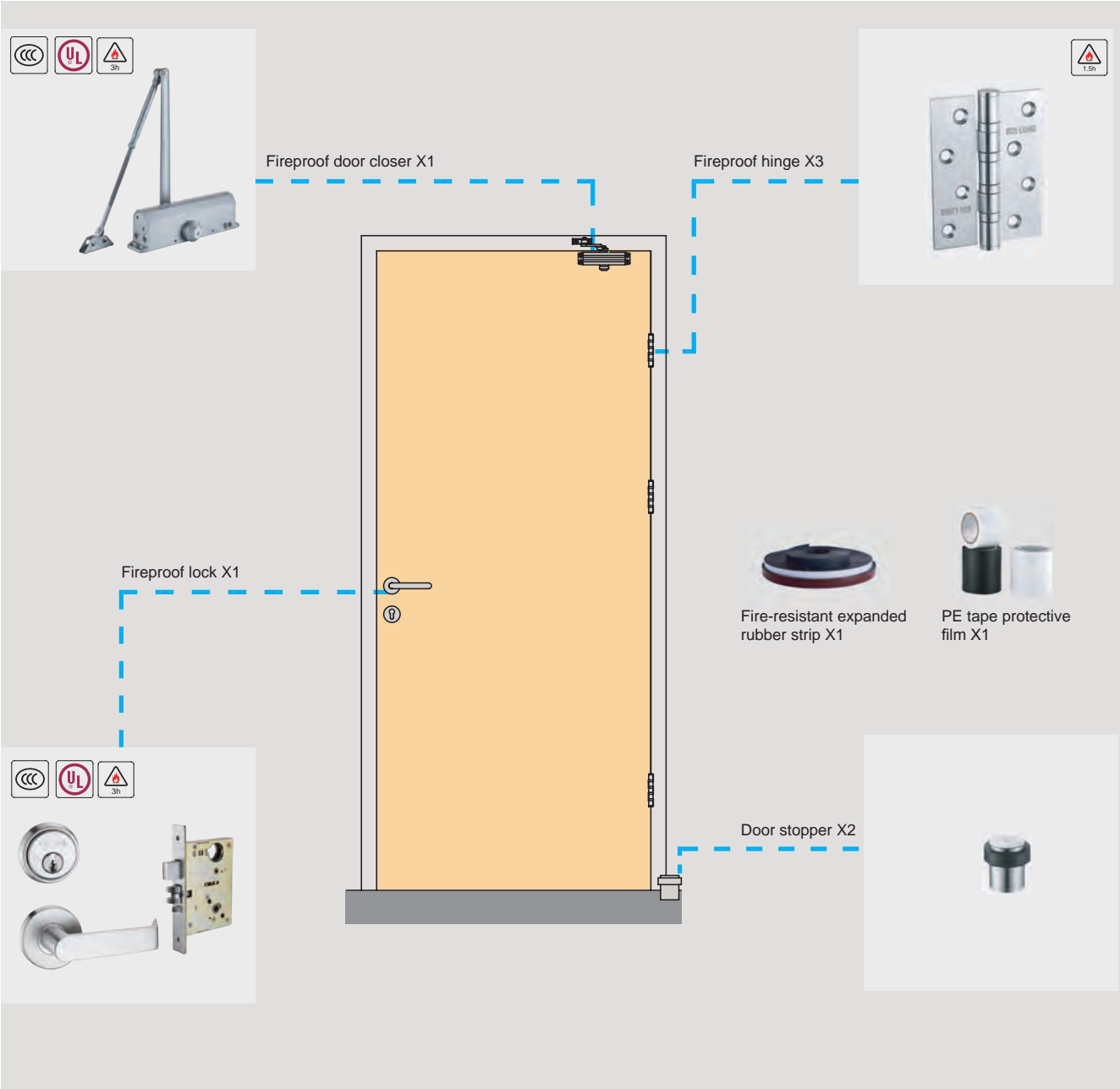
Single-opening fireproof doors configuration scheme
