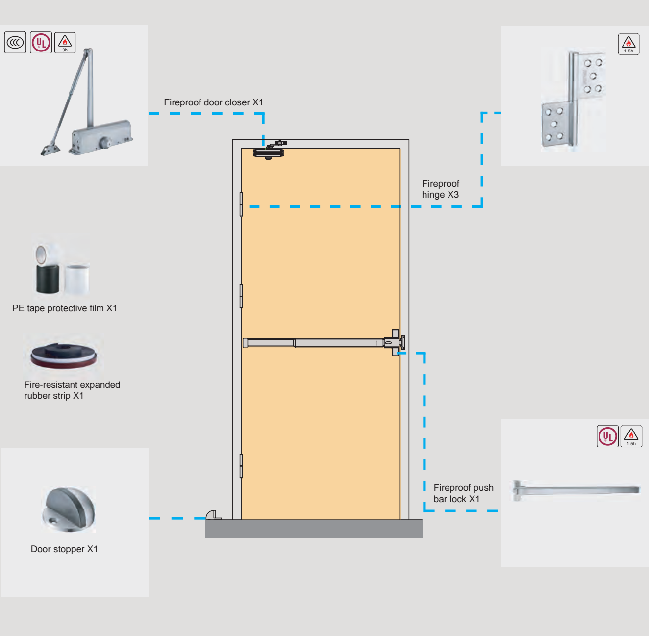
Single-opening escape fireproof doors configuration scheme
