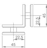
WWB31030 Original Code: WB3103 Glass Door Thickness: 8-10mm
