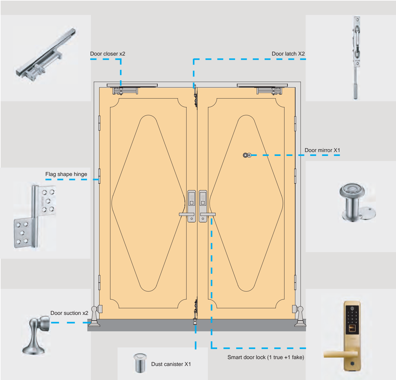
Double-opening entrance doors configuration scheme
