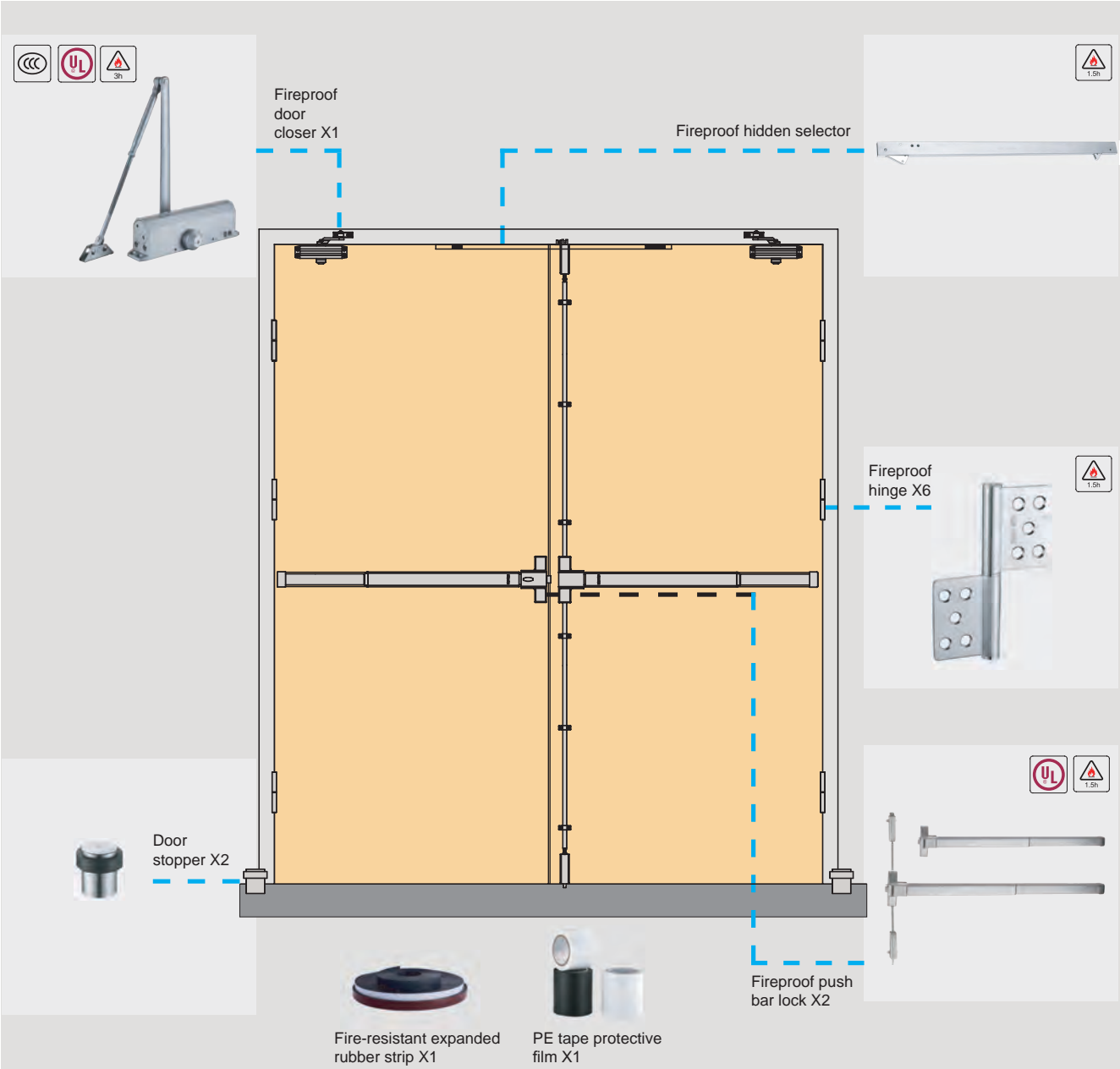
Double-opening escape fireproof doors configuration scheme
