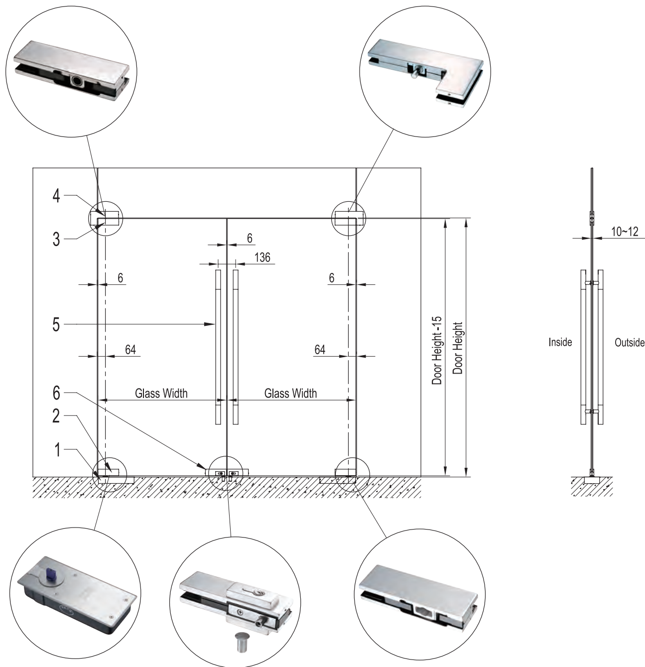
Configuration of Frameless Glass Door with Floor Hinge
