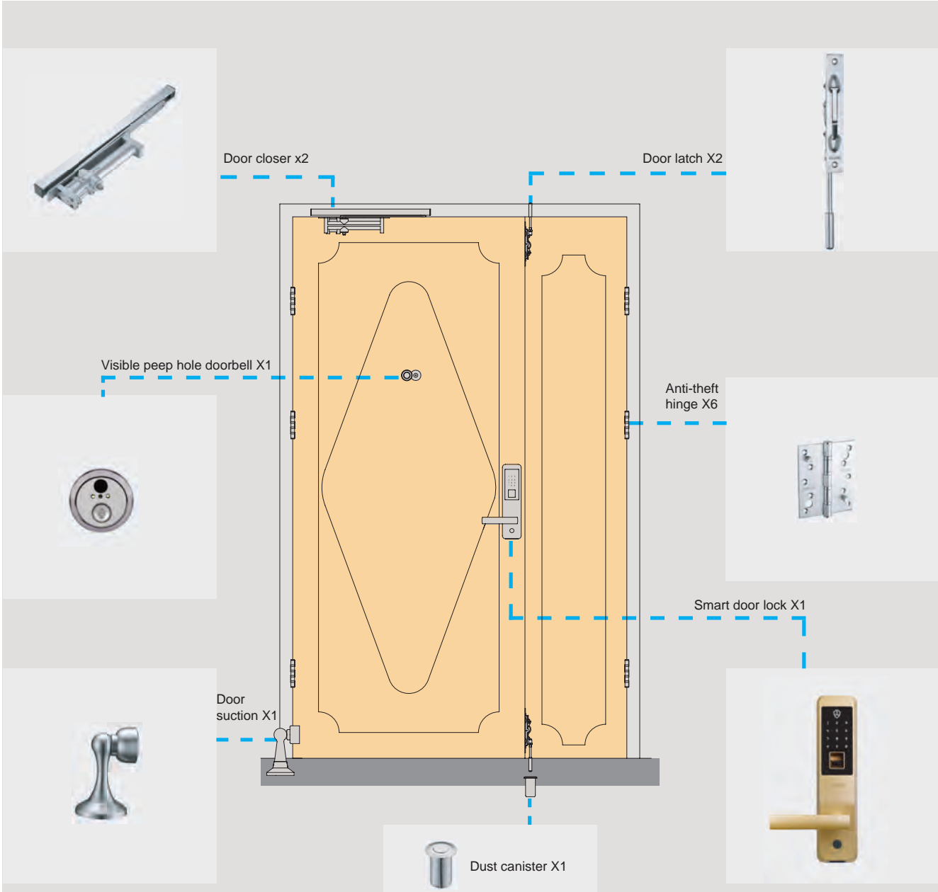
Unequal double doors configuration scheme
