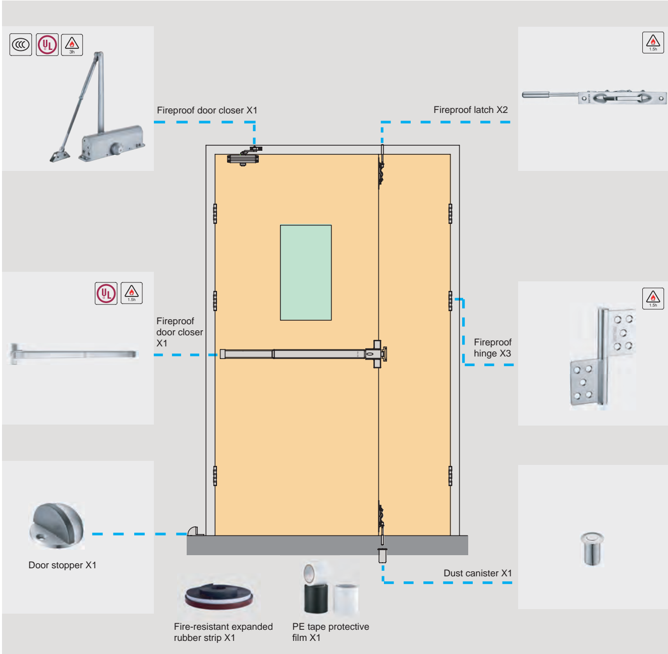
Unequal escape fireproof doors configuration scheme
