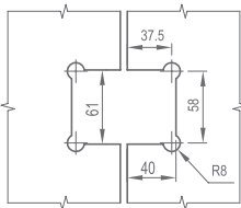
WHY11050 Original Code: Y1105
