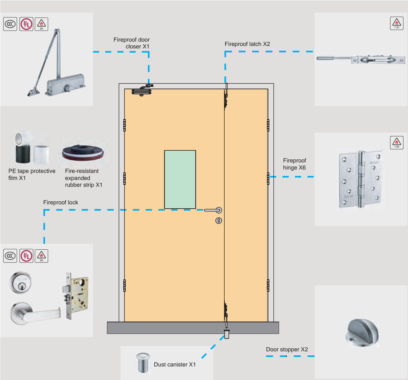
Unequal fireproof doors configuration scheme
