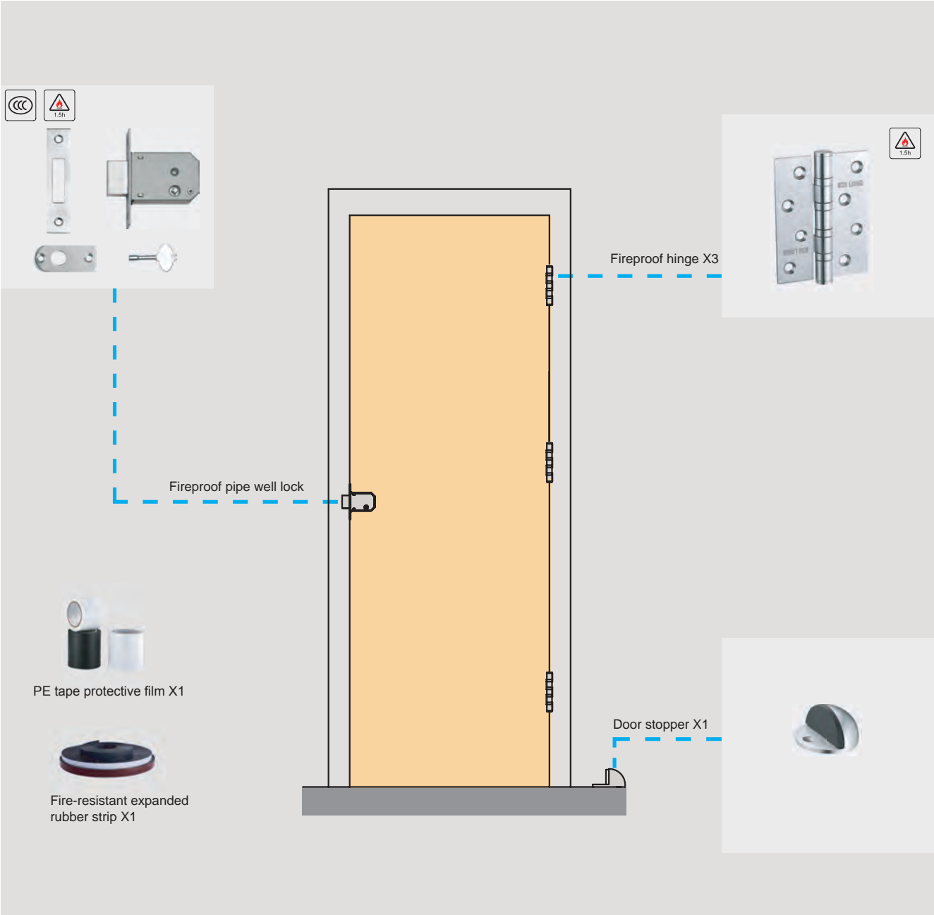
Pipe well door doors configuration scheme
