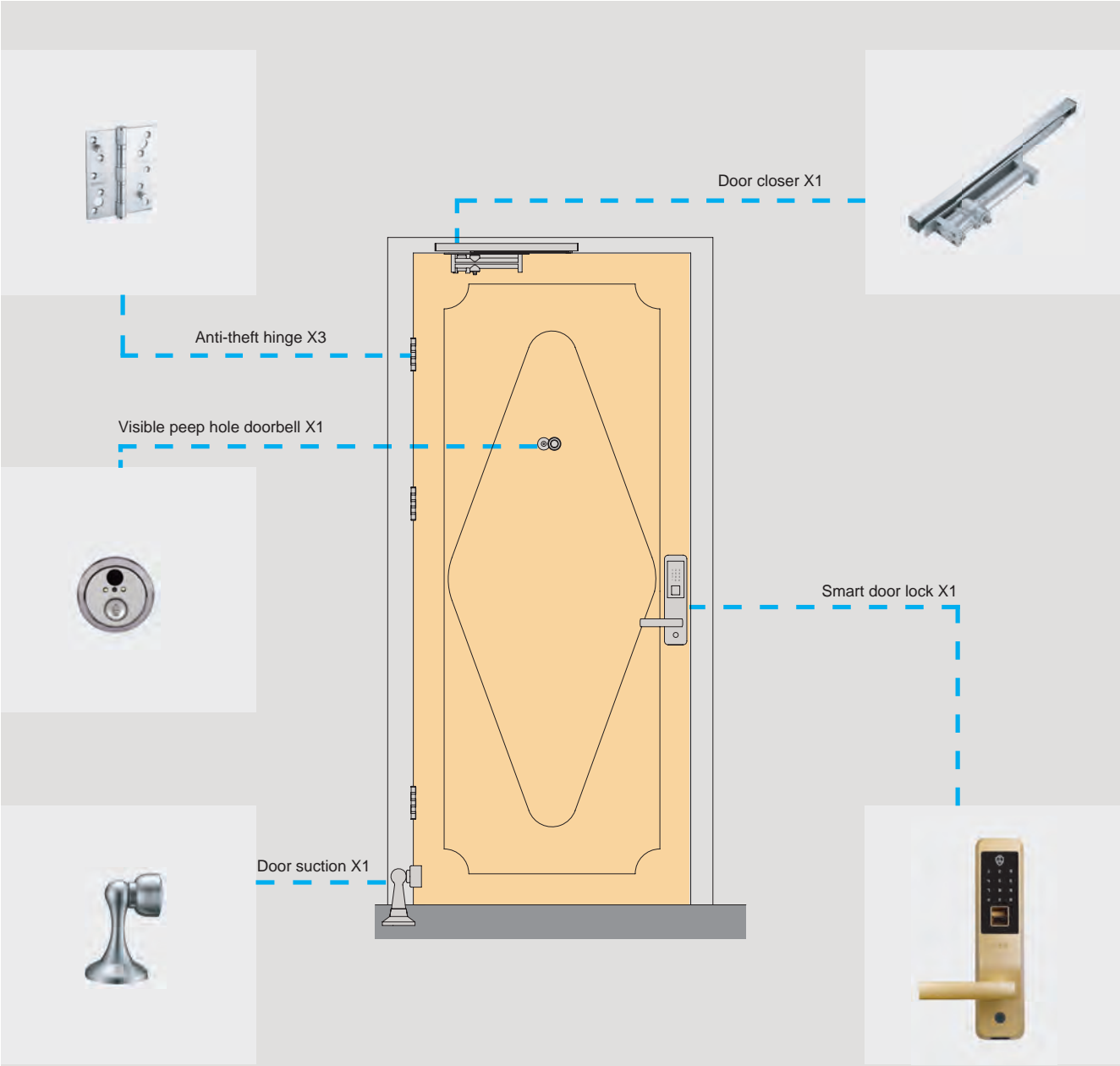
Single-opening entrance doors configuration scheme
