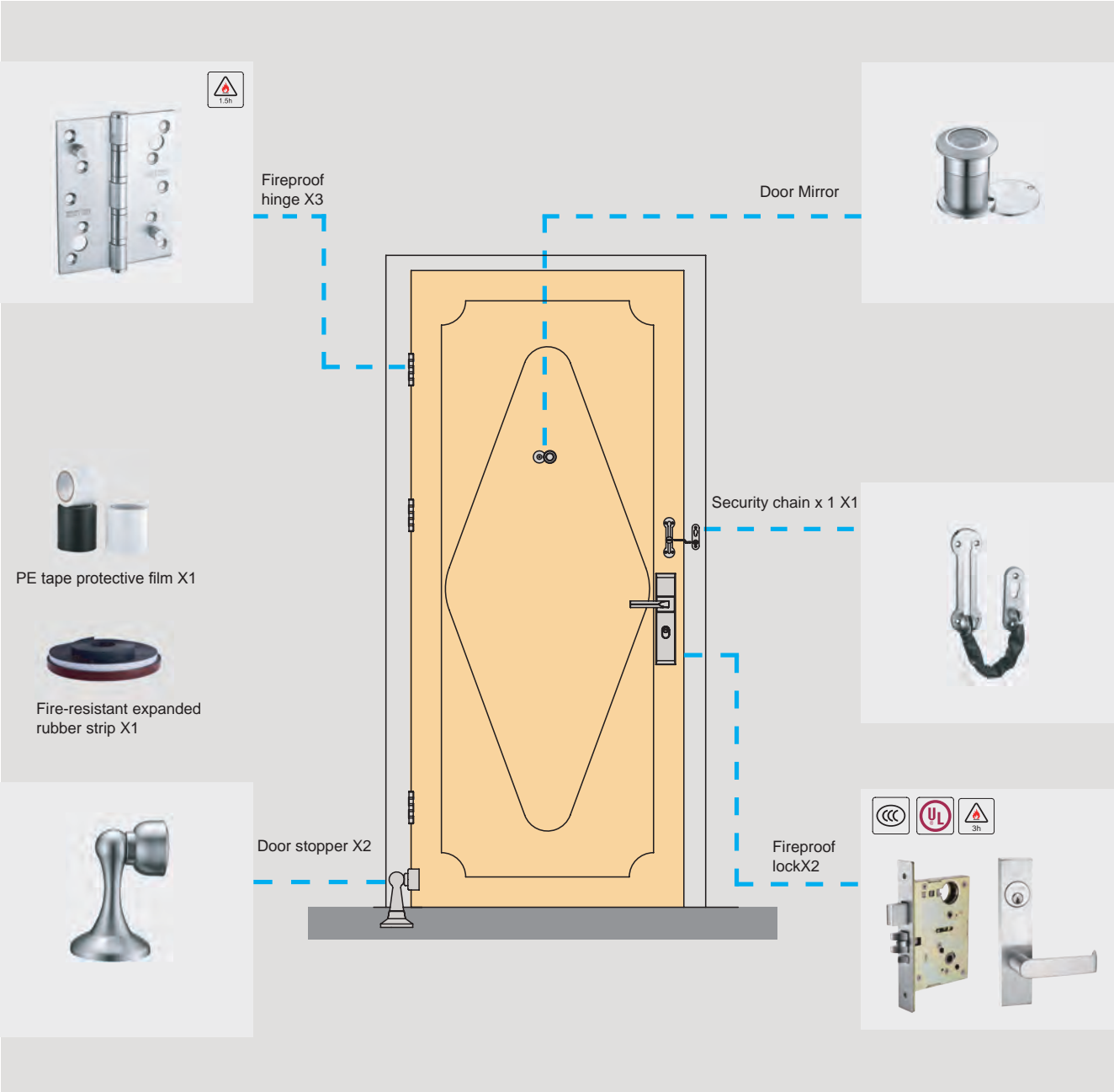
Anti-theft fire doors configuration scheme
