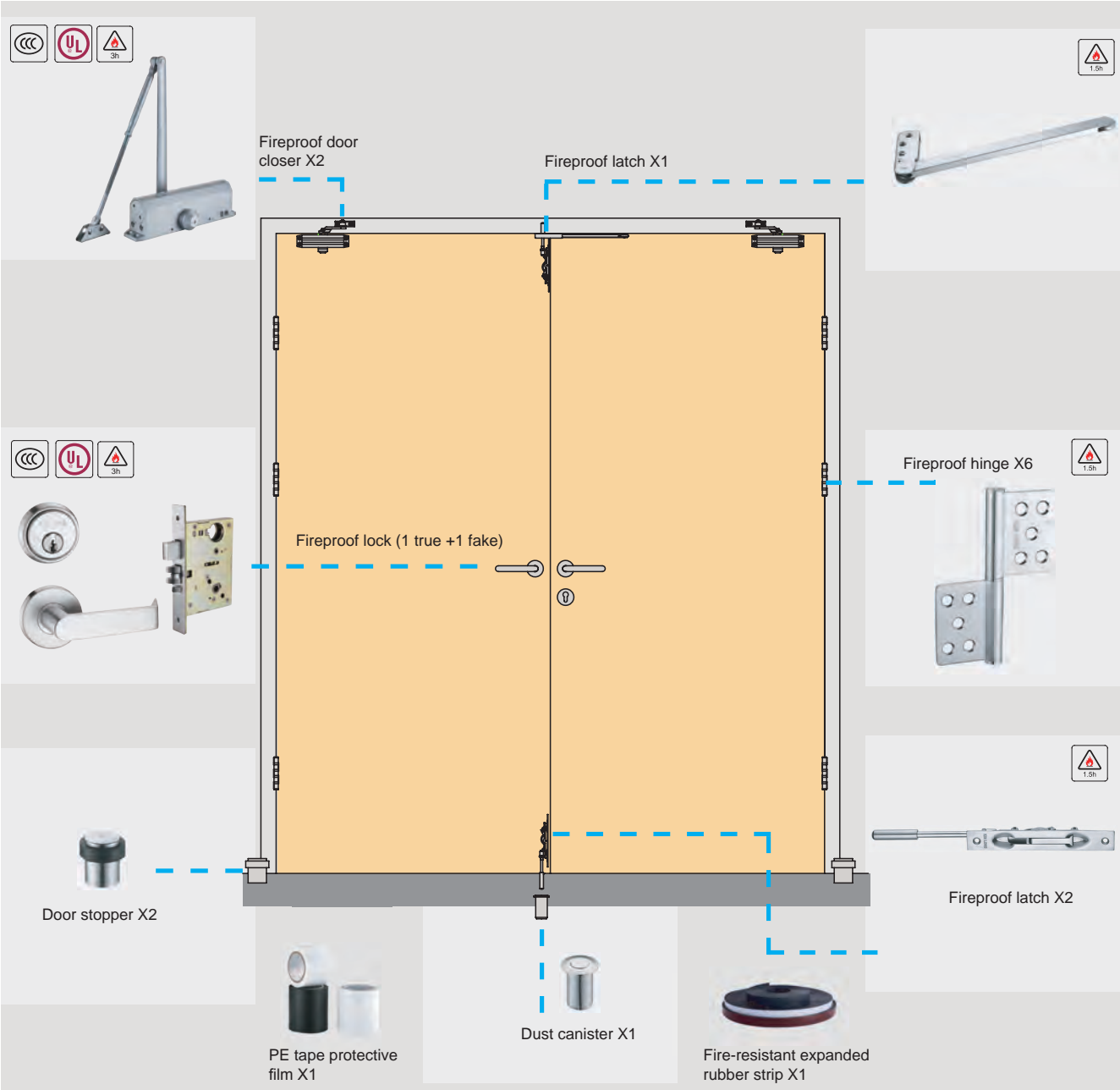
Double-opening fireproof doors configuration scheme
