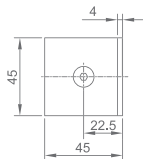
WWB31010 Original Code: WB3101 Glass Door Thickness: 8-10mm
