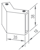
WTL10090 Original Code: YTL109 Product Name: 135° Connector
