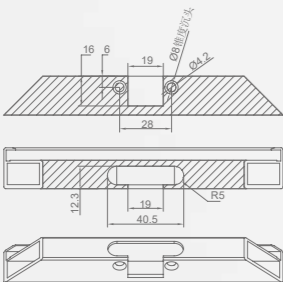
Profile hole drawing
