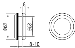
T1L03 暗拉手 Concealed handle
