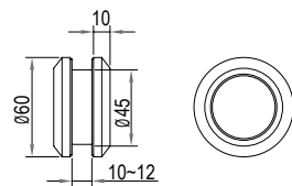
T1L04 暗拉手 Concealed handle
