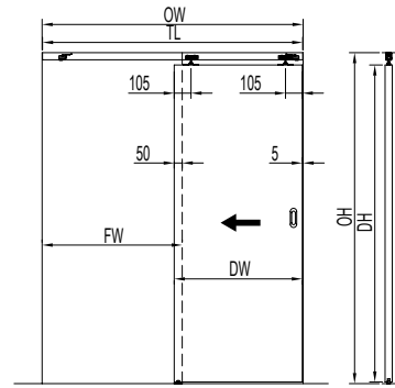
T1L13 暗拉手 Concealed handle
