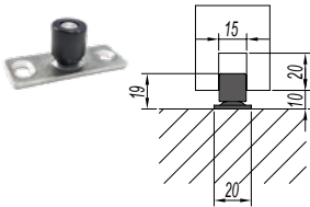
门底导向件开孔图 Swing stopper Opening Hole
