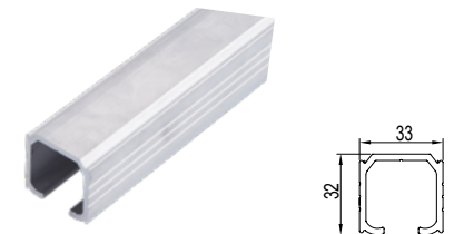
T3G90 吊轨 Hanging Rail
