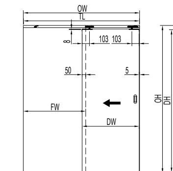
T1L12 暗拉手 Concealed handle
