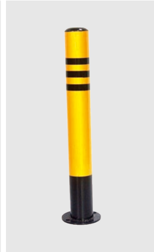
Name: Protective Pile (Fixed) Model: TLJT-FHZ01 Specification: \phi 76 \times 600 \text{mm} \phi 89 \times 750 \text{mm} , \phi 114 \times 1000 \text{mm} Material: high quality steel pipe, high pressure spraying Engineering grade reflective film Application: road entrance
