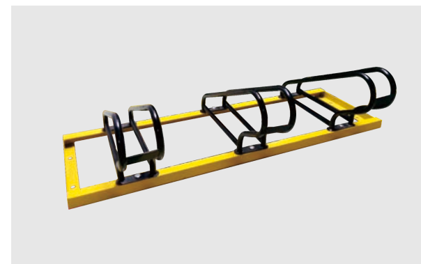
Name:Bicycle rack Specification:1200X550X300mm Material:High-temperature steel spraying Model:TLJT-ZXC-J01 Application:Schools and other public places
