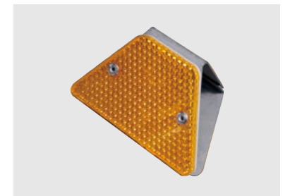
Name: Trapezoidal contour marker Model: TLJT-LLB02-T Specification: 120 \times 80 \text{mm} Application: parking lot, road
