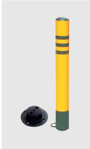
Name: Protective Pile (Activity) Model: TLJT-FHZ02 Specification: \phi 76 \times 600 \text{mm} \phi 89 \times 750 \text{mm} , \phi 114 \times 1000 \text{mm} Material: high quality steel pipe, high pressure spraying Engineering grade reflective film Application: road entrance
