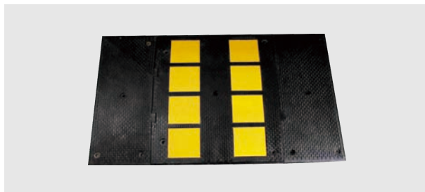
Name: Reflective deceleration slope Model: TLJT-JSP12 Specifications: 470X600X35mm Material: rubber Application: hospital, road
