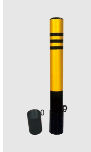
Name: Protective Pile (Activity) Model: TLJT-FHZ02-M Specification: \phi 76 \times 600 \text{mm} \phi 89 \times 750 \text{mm} , \phi 114 \times 1000 \text{mm} Material: high quality steel pipe, high pressure spraying Engineering grade reflective film Application: road entrance
