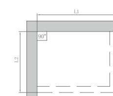
Measure wall side size without stone base
