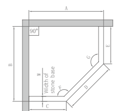
Angle measurement under embedded stone base situation
