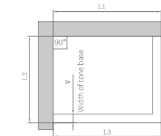
Embedded stone base and wall angle is in 90 degree
