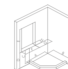
Length measurement under embedded stone base situation
