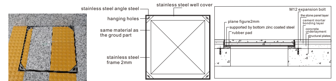
Stainless steel well cover
